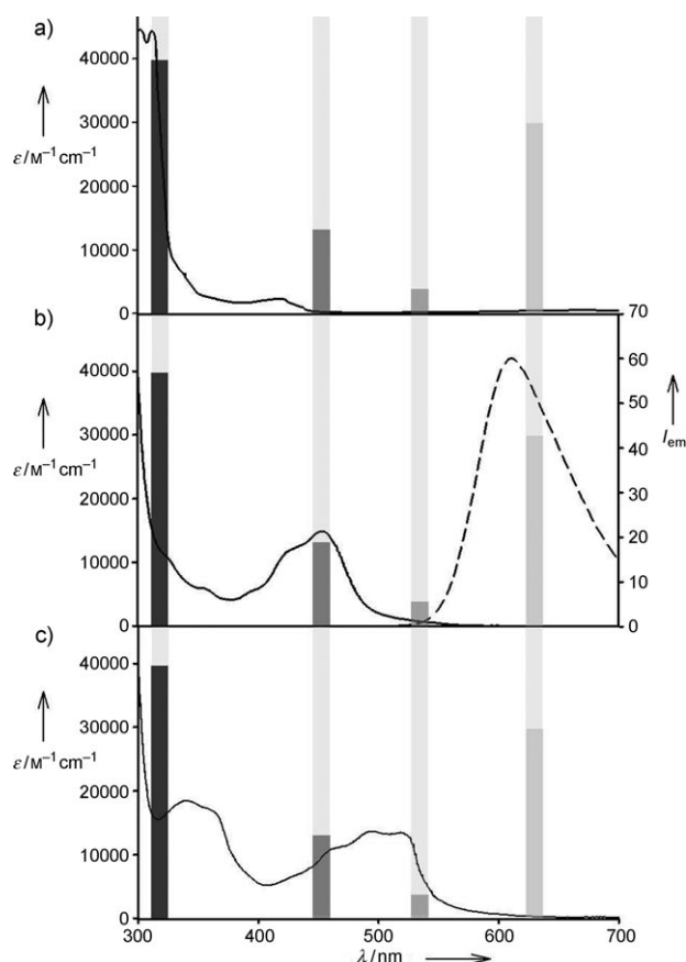
Figure 3. Absorption and emission spectra of [\text{Ru}(\text{bpy})_3]^{2+} (b), and its oxidized [\text{Ru}(\text{bpy})_3]^{3+} (a) and reduced [\text{Ru}(\text{bpy})_3]^{+} (c) species. The shaded rectangles indicate the chosen value of the thresholds for encoding/decoding operations.
